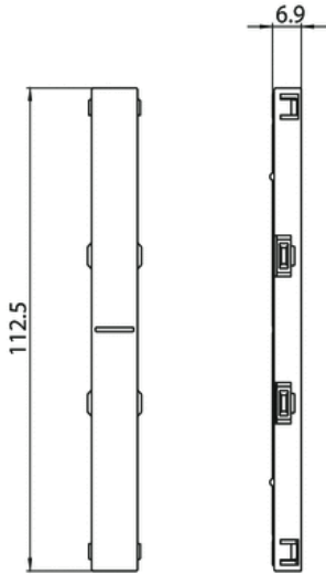
BLOKINLINE 180° UNION
