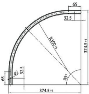
BLOKINLINE PROFILE R300-R500
