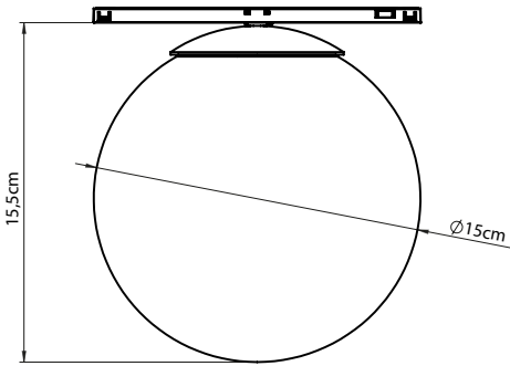
BLOKINLINE SPHERE 150
