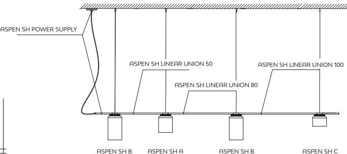
ASPEN SH INSTALLATION EXAMPLE
