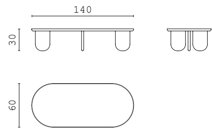
CALIPSO 140 coffee table
